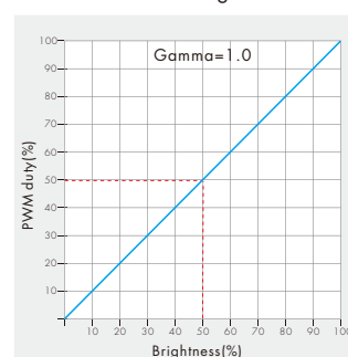
Linear dimming curve
